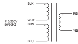
Schematic 3
